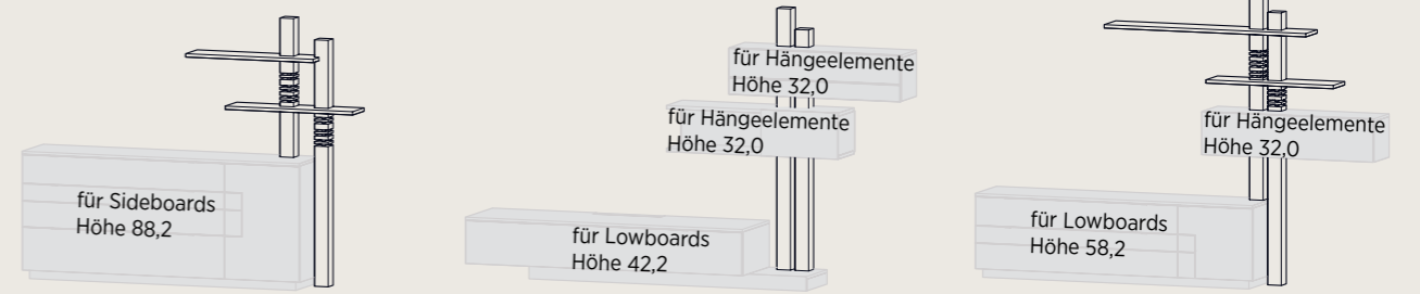
SIG-201130* B 121,6 | H 184,0 | T 23
